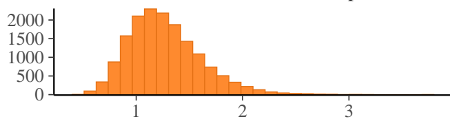
sd_lex__mudirhe_Intercept
