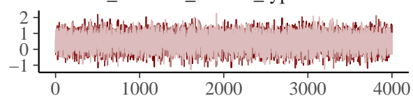
b_mudirhe_motion_typeeffective
