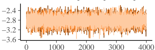
b_mudirhe_cmpl_complexcomplex
