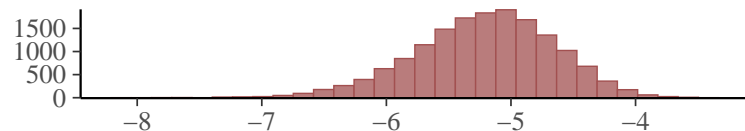
b_mudirhe_cmpl_animanim
