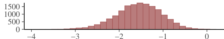
b_mvuc_verse_genreinstruction
