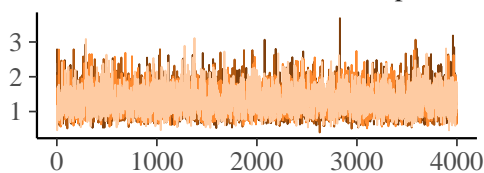
sd_lex__mudirhe_Intercept
