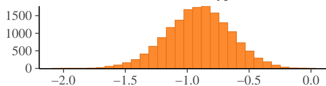
b_mudirhe_motion_typefictive
