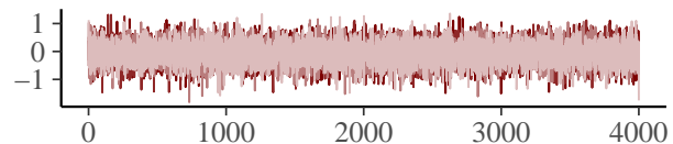
b_mvuc_motion_typefictive
