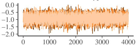
b_mudirhe_motion_typefictive
