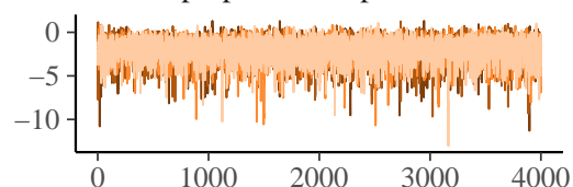
b_muprekdirhe_cmpl_animanim
