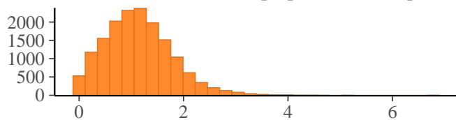
sd_book_scroll__muprepdirhe_Intercept
