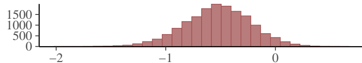
b_mudirhe_Intercept
