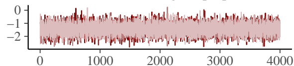
b_mudirhe_verse_genreprophetic
