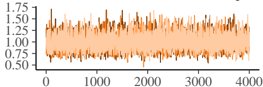
sd_book_scroll__muvc_Intercept
