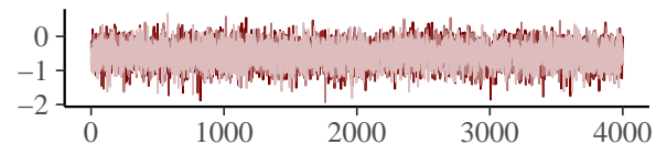
b_mudirhe_Intercept
