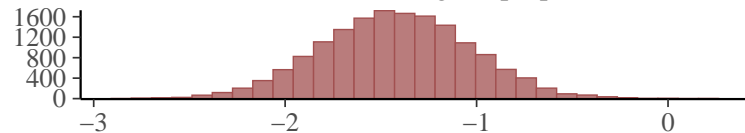
b_mudirhe_verse_genreprophetic
