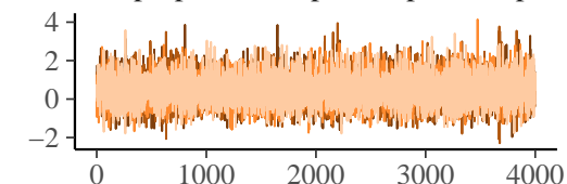
b_muprekdirhe_cmpl_complexcomplex
