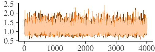
sd_book_scroll__mudirhe_Intercept
