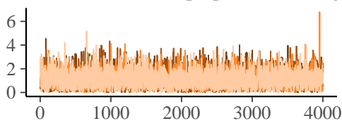
sd_book_scroll__muprepdirhe_Intercept
