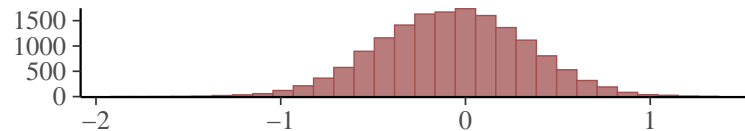
b_mvuc_motion_typefictive
