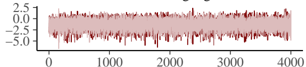
b_muvc_verse_languageAramaic
