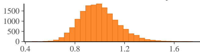
sd_book_scroll__muvc_Intercept
