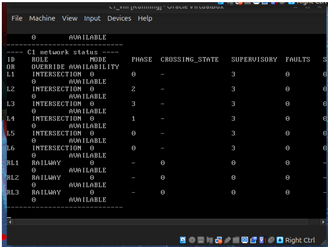
Figure 12. 45-second approach warning, boom gate closure, and confirmation-before-proceed train signal interlock (2)
