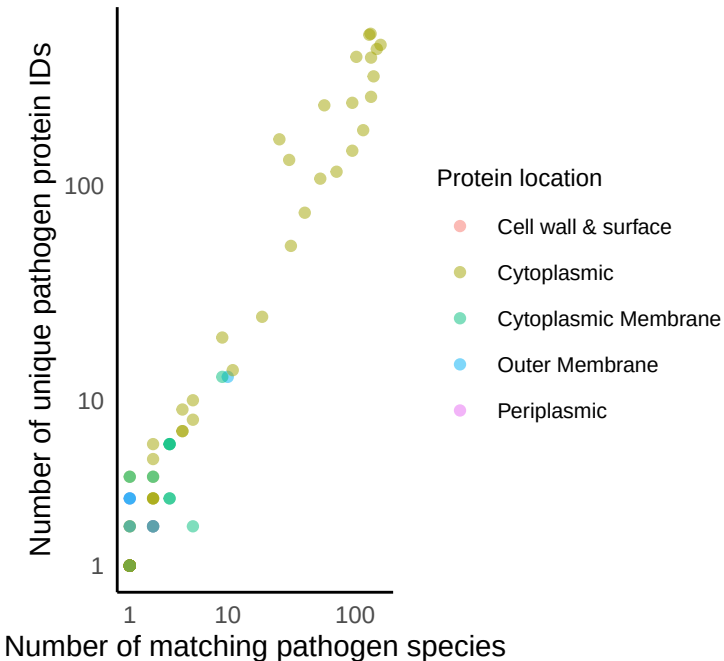
A. Pathogen protein subcellular location
