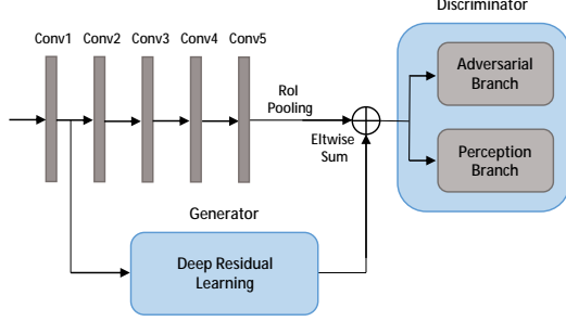
Figure 2. Training procedure of object detection network based on the Perceptual GAN. The perception branch of the discriminator network along with the bottom convolutional layers is first trained using the training images that contain only large objects. Then with the training images that contain only small objects, the generator network is trained to generate super-resolved large-object like representations for small objects. The adversarial branch of the discriminator network is trained to differentiate between the generated super-resolved representations for small objects and the original ones for real large objects. By iteratively boosting the abilities of the generator network and the discriminator network through alternative training, the detection accuracy especially for small objects can be improved.
