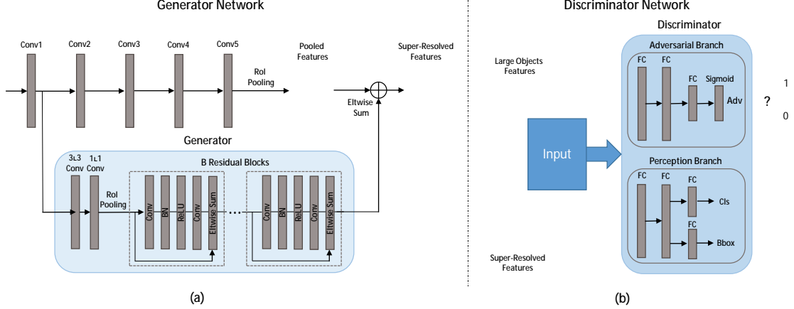
Figure 3. Details of the proposed Perceptual Generative Adversarial network. (a) The generator is a deep residual network which takes the features with fine-grained details from lower-level layer as input and passes them to 3 \times 3 convolutional filters followed by 1 \times 1 convolutional filters to increase the feature dimension to be aligned with that of “Conv5”. Then B residual blocks each of which consists of convolutional layers followed by batch normalization and ReLU activation are employed to learn the residual representation, which is used to enhance the pooled features from “Conv5” for small objects to super-resolved representation through element-wise sum operation. (b) The discriminator takes the features of large object and the super-resolved representation of small object as inputs and splits into two branches. The adversarial branch consists of three fully connected layers followed by sigmoid activation, which is used to estimate the probability that the current input representation belongs to that of real large object. The perception branch consists of two fully connected layers followed by two output sibling layers, which are used for classification and bounding box regression respectively to justify the detection accuracy benefiting from the generated super-resolved representation.
