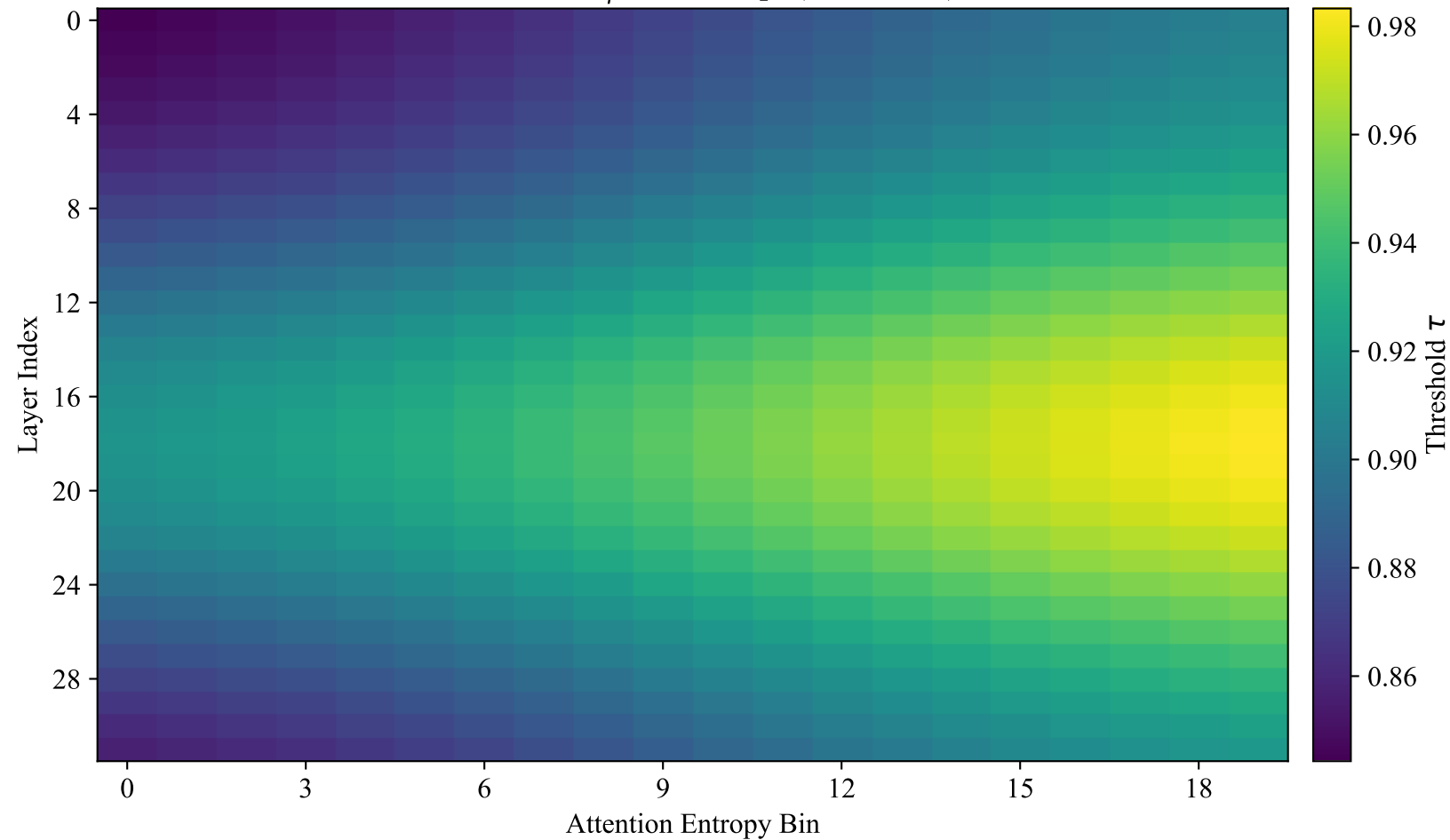
M_{\text{lex}}(l, b_h, b_p) Heatmap (PPL Bin 0)
