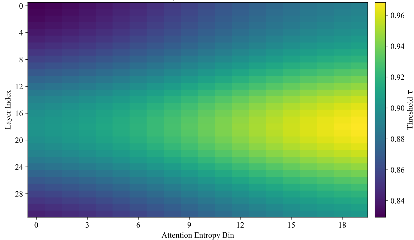
M_{\text{lex}}(l, b_h, b_p) Heatmap (PPL Bin 1)
