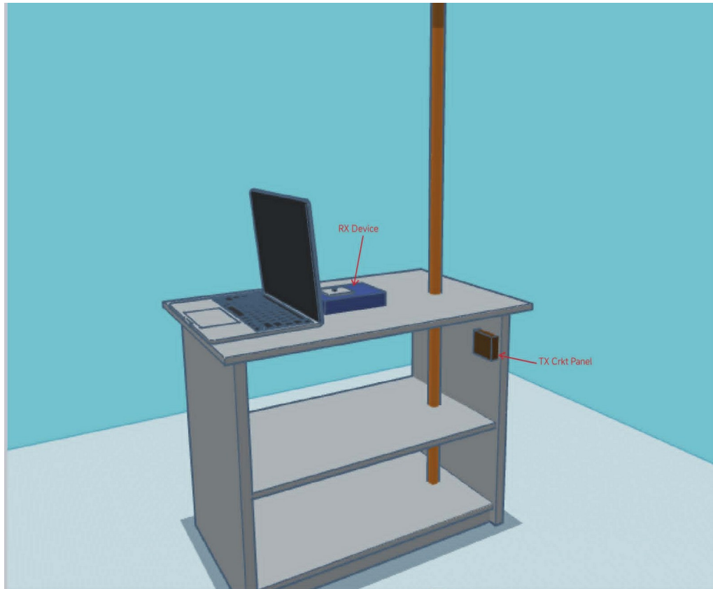
Figure 3.24.. RX Setup 3D Model Close-up view
