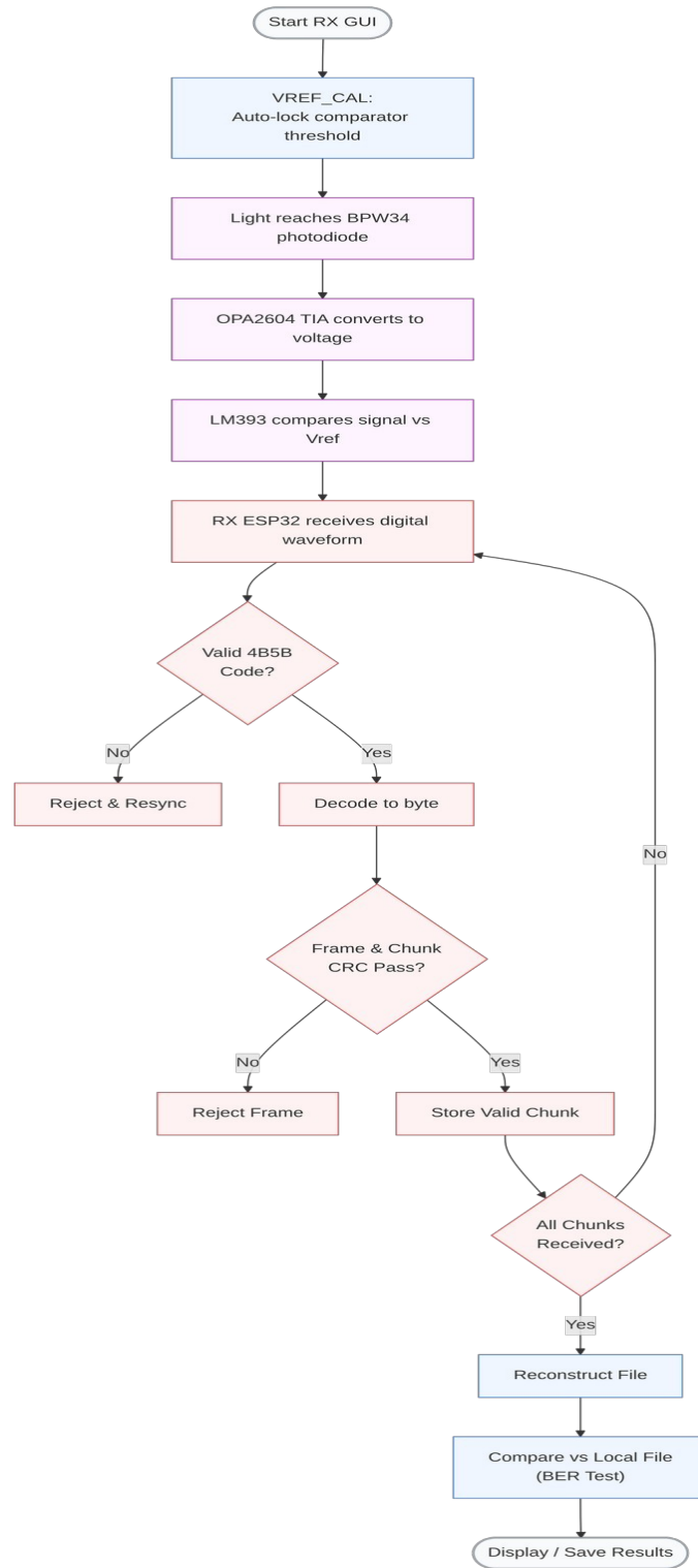
Figure 3.20. Receiver Flow System
