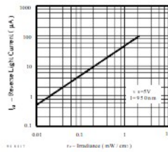
Figure 3. Reverse Light Current vs. Irradiance
