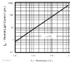
Figure 4. Reverse Light Current vs. Illuminance
