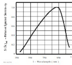
Figure 7. Relative Spectral Sensitivity vs. Wavelength
