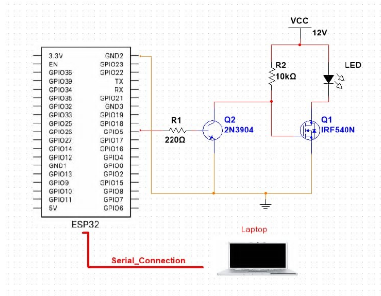
Figure 3.21. Transmitter Schematic Diagram
