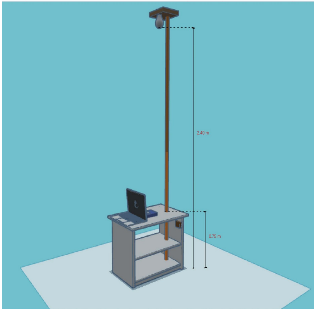
Figure 3.23. Prototype 3D Model with measurements
