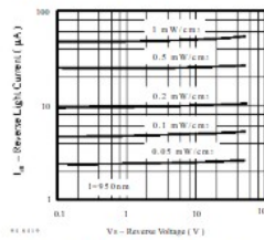
Figure 5. Reverse Light Current vs. Reverse Voltage
