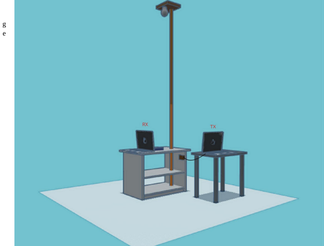
3.25. 3D Model of the RX/TX system setup
