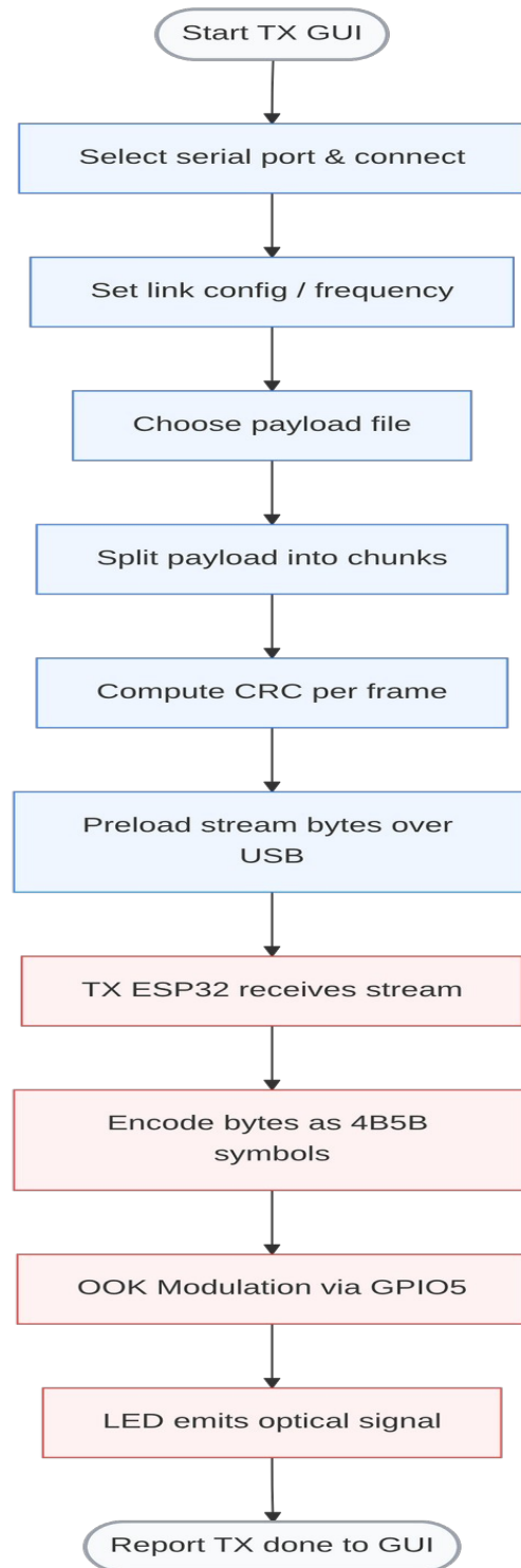
Figure 3.19. Transmitter Flow System
