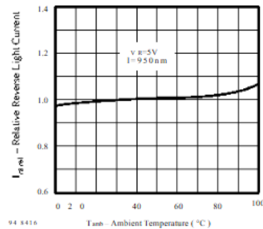
Figure 2. Relative Reverse Light Current vs. Ambient Temperature
