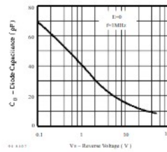
Figure 6. Diode Capacitance vs. Reverse Voltage
