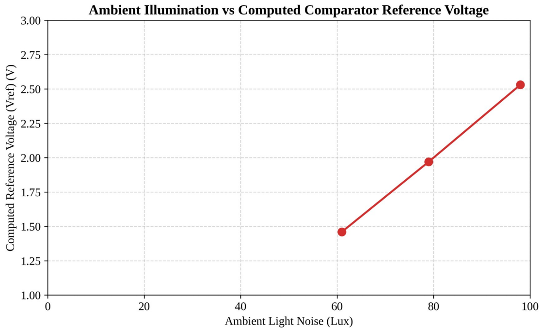
Figure 4.6. Ambient Illumination vs Computed Comparator Reference Voltage
