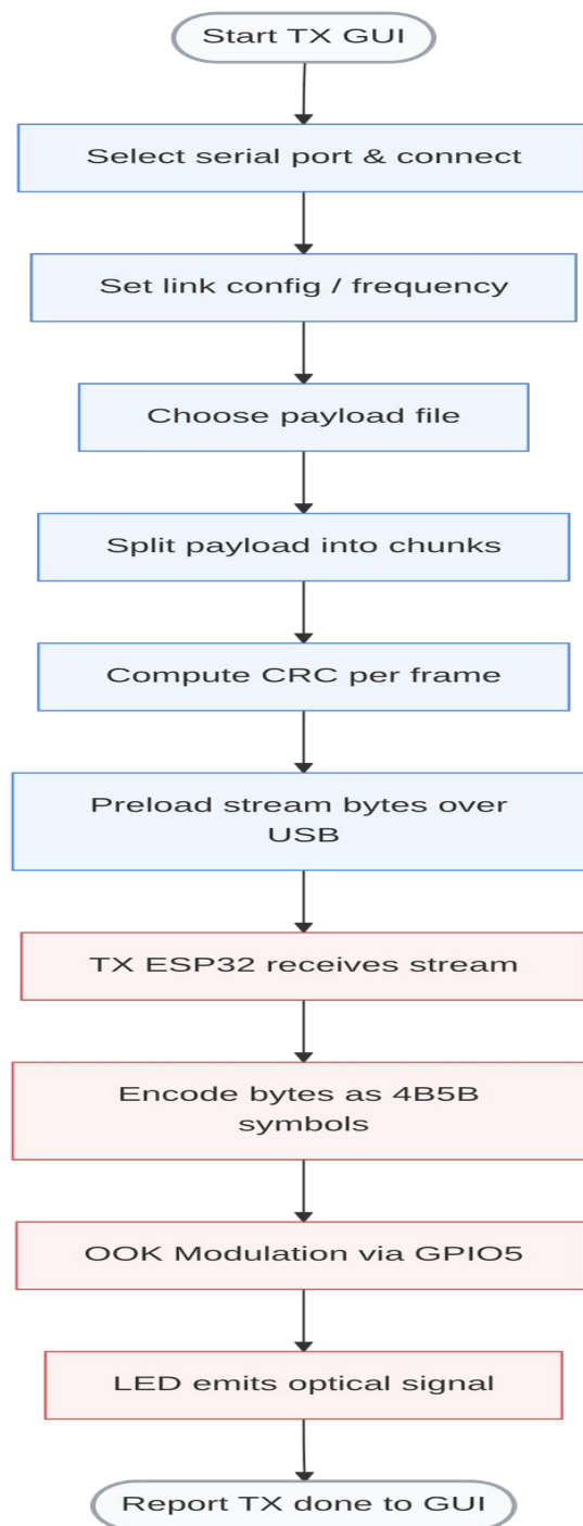
Figure 3.3.2. Transmitter Flow System
