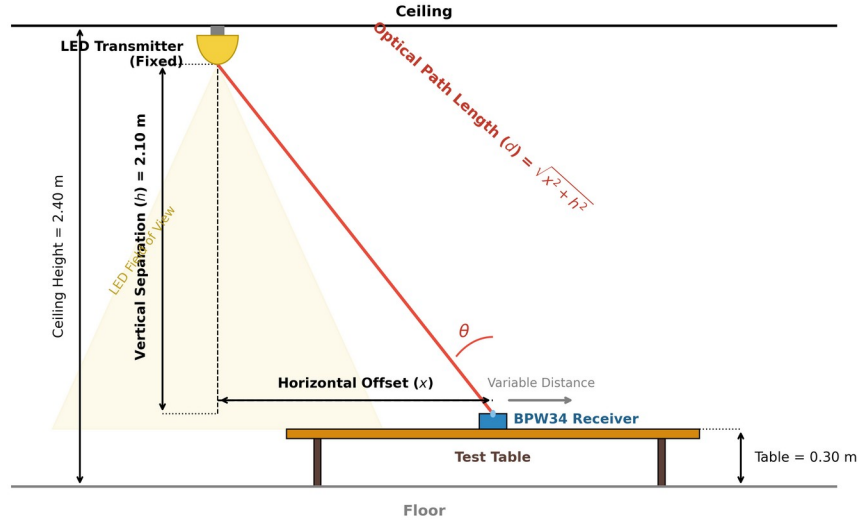
Figure 3.1.1. Experimental setup geometry and resulting optical path length.
