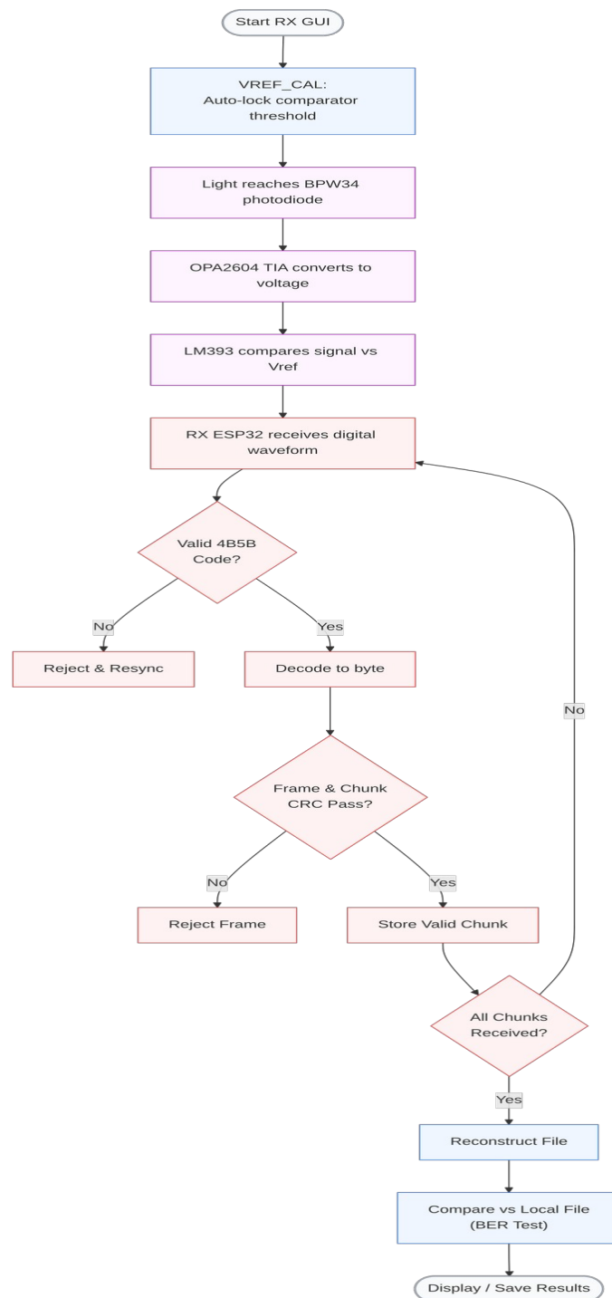
Figure 3.3.3 Receiver Flow System
