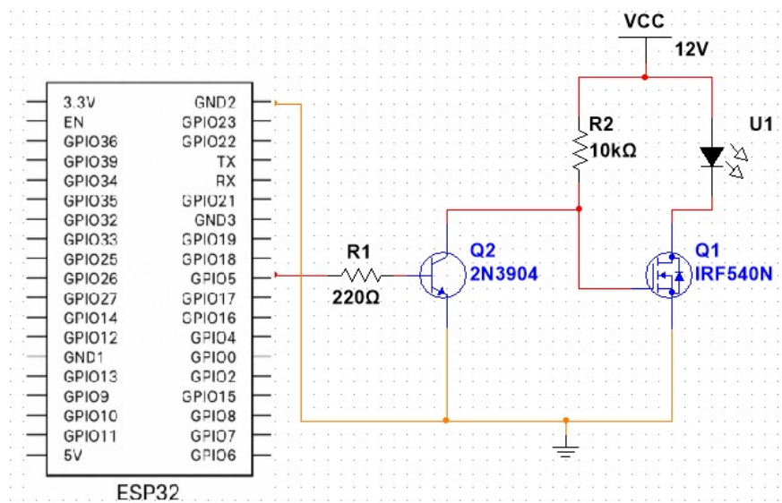
Figure 3.4.1 Transmitter Schematic Diagram
