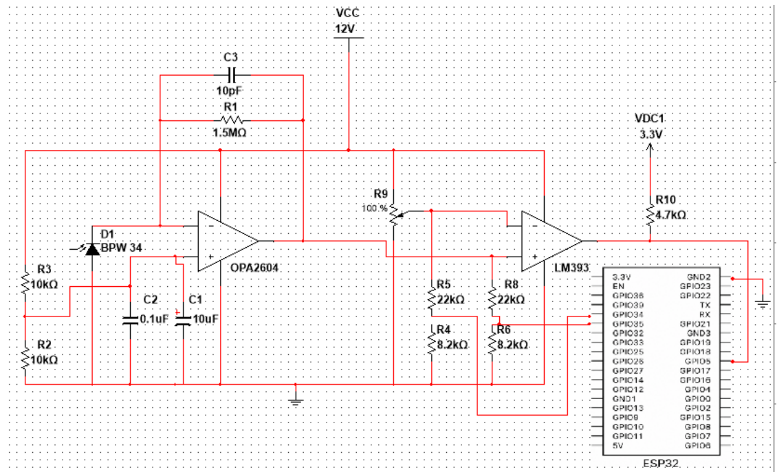
Receiver Schematic Diagram
