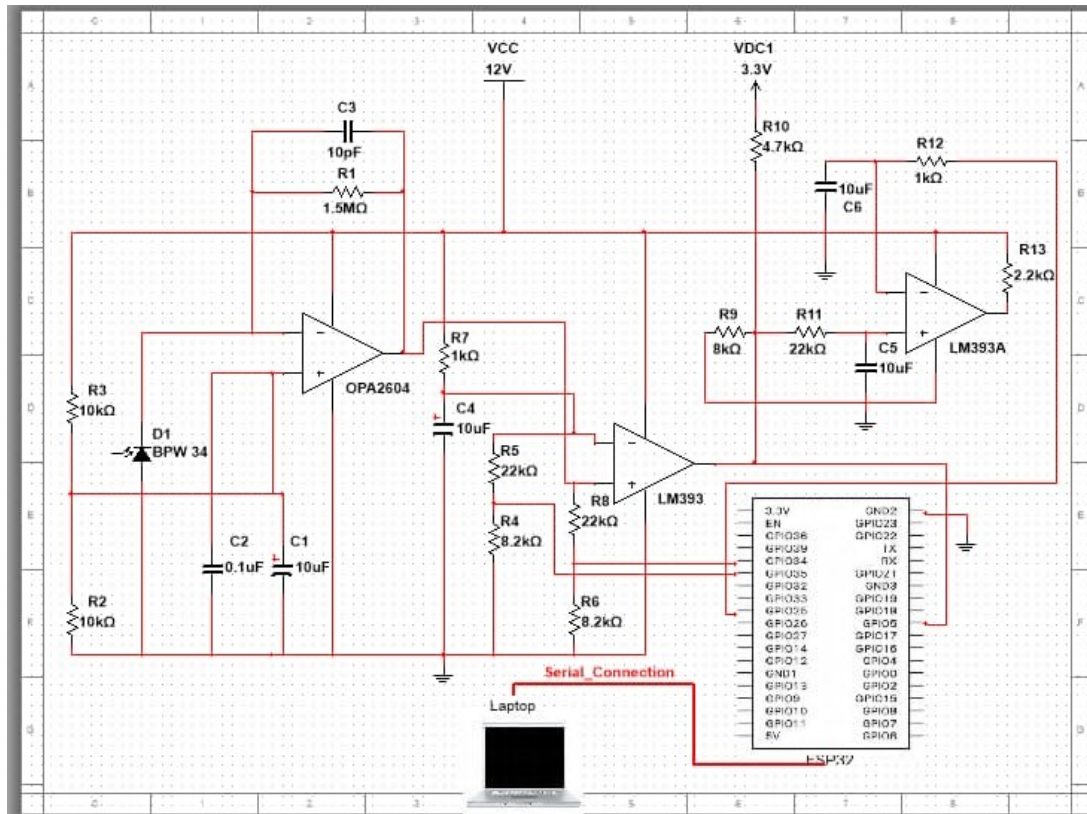
Figure 3.23. Receiver Schematic Diagram
