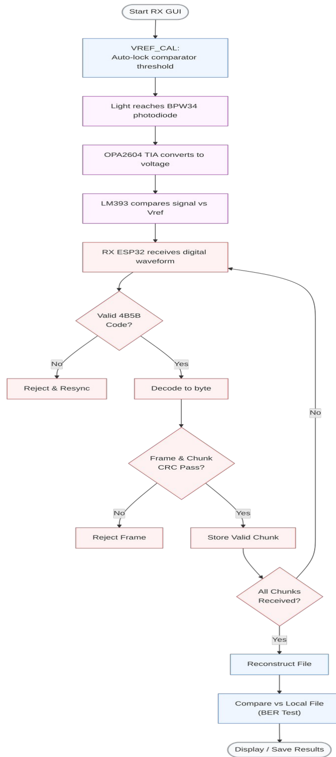
Figure 3.21. Receiver Flow System
