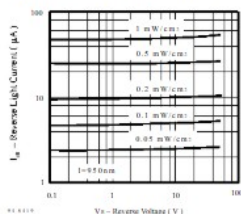
Figure 5. Reverse Light Current vs. Reverse Voltage
