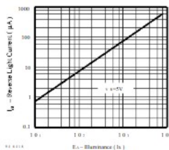
Figure 4. Reverse Light Current vs. Illuminance
