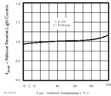
Figure 2. Relative Reverse Light Current vs. Ambient Temperature
