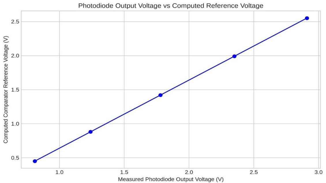
Figure 4.1. Measured Photodiode Voltage vs Computed Comparator Reference Voltage
