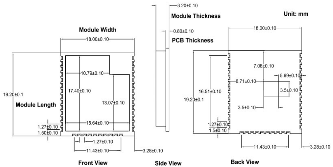
Dimentions Diagram
