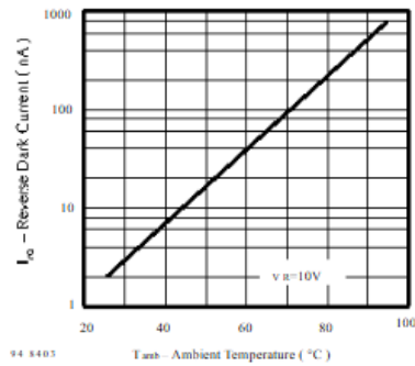
Figure 1. Reverse Dark Current vs. Ambient Temperature
