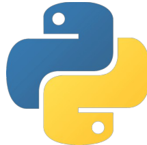
Figure 3.14 Python v13.14.5
