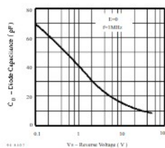
Figure 6. Diode Capacitance vs. Reverse Voltage
