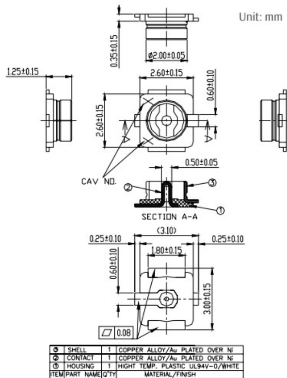
UFL Dimensions Diagram
