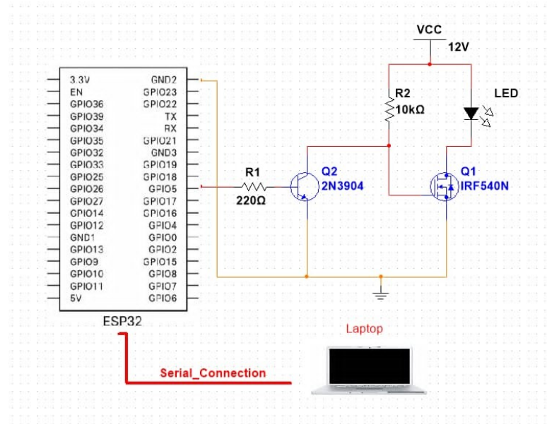
Figure 3.22. Transmitter Schematic Diagram
