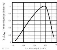
Figure 7. Relative Spectral Sensitivity vs. Wavelength
