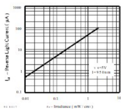
Figure 3. Reverse Light Current vs. Irradiance
