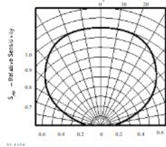
Figure 8. Relative Radiant Sensitivity vs. Angular Displacement
