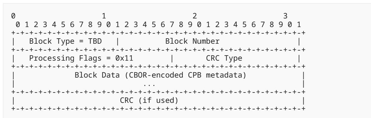
Figure 1: Bundle Extension Block Format (Octet Diagram)
