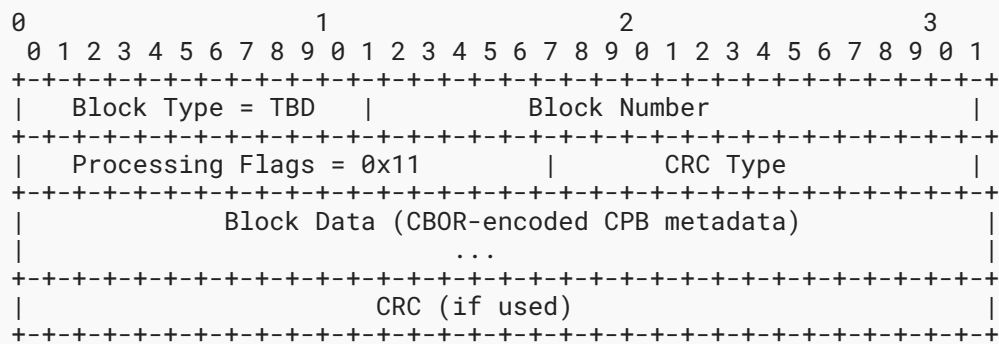
Figure 1: Bundle Extension Block Format (Octet Diagram)
