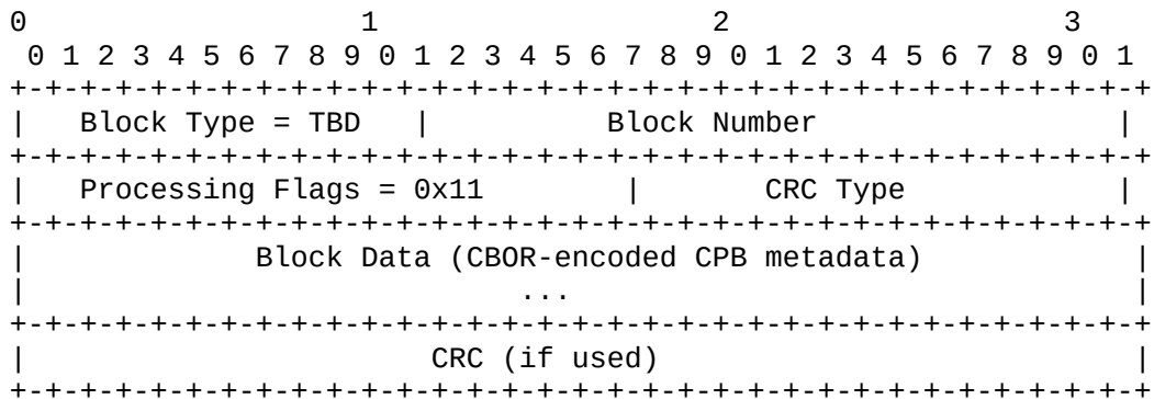
Figure 1: Bundle Extension Block Field Order (Schematic)
