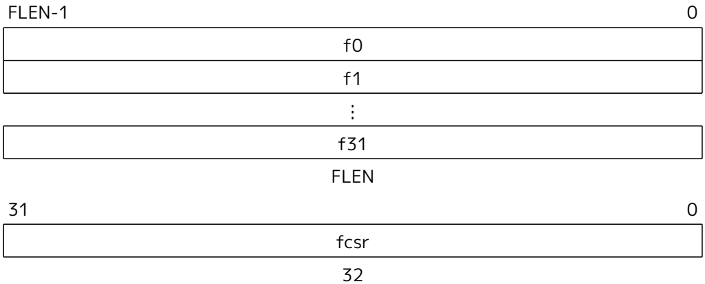
Figure 3. RISC-V floating-point register state
