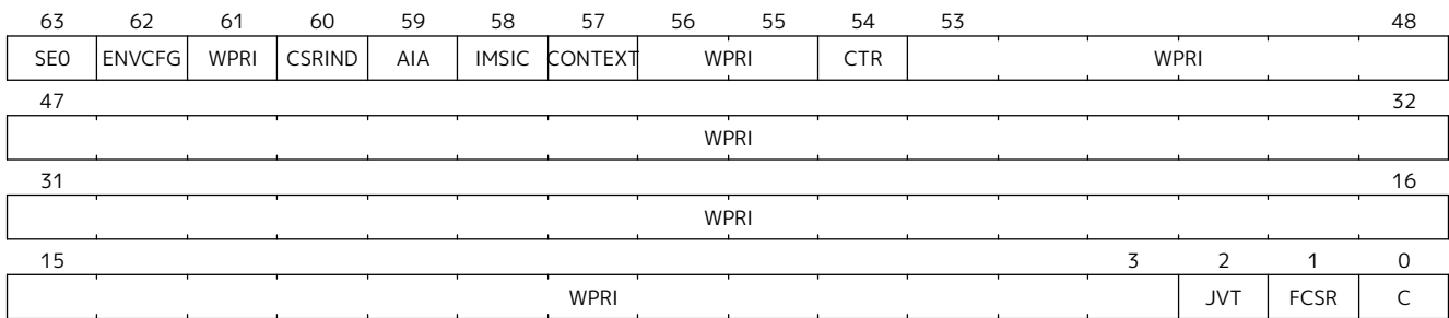
Figure 119. Hypervisor State Enable 0 Register ( hstateen0 )
