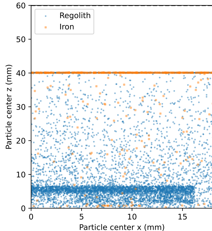
FIG. 3 — Good-variable DEM checkpoint Historical filename: real drag, 1.5 mm iron, gas input 3.5 m/s
