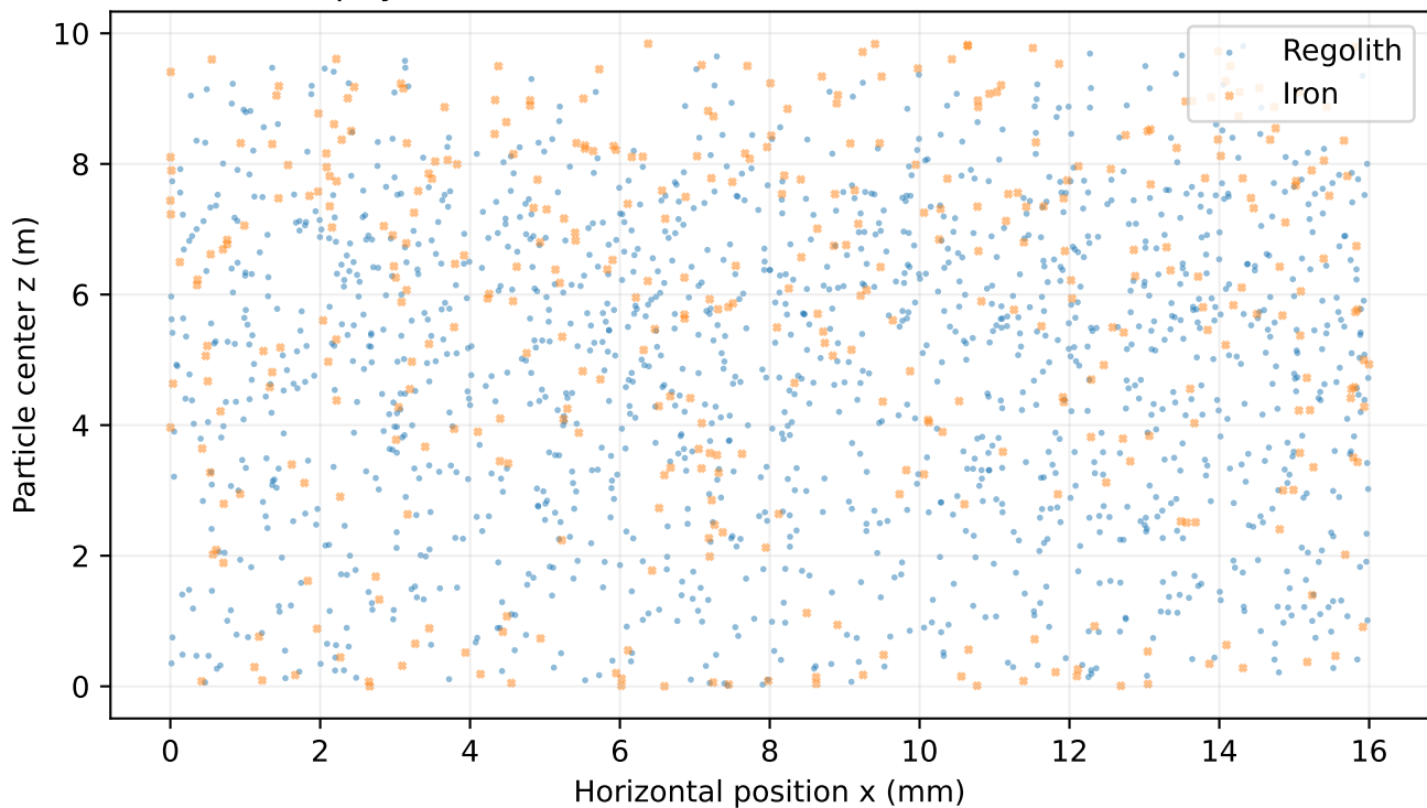
FIG. 3 — Historical Rung 5 checkpoint, step 200,000 No physical lid: not evidence of a confined fluidized bed
