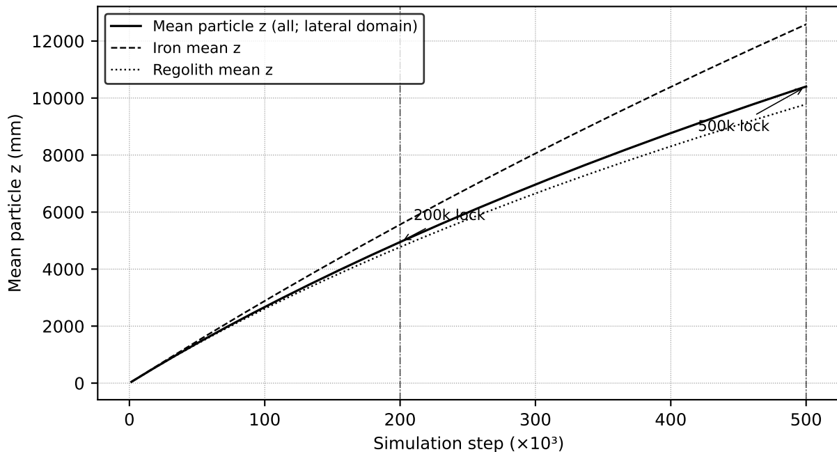
FIG. 7 — Rung 5 sensitivity GPU DEM mobilization progression Historical no-lid run: lateral containment only; not physical bed-height evidence
