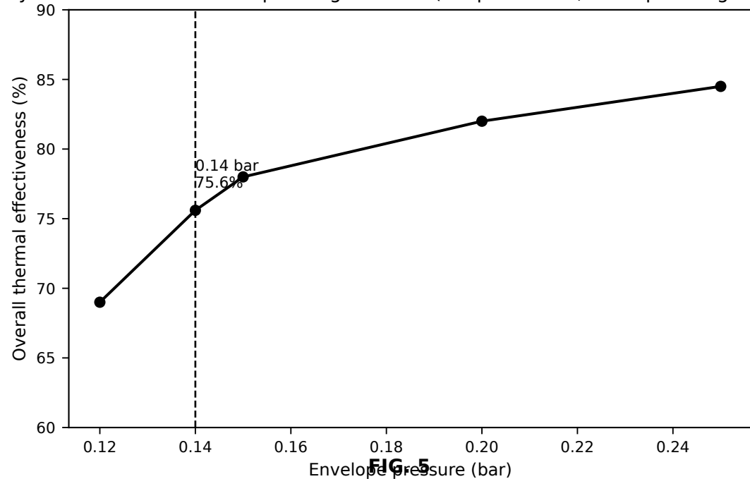
System Effectiveness vs. Operating Pressure (lumped model, claim point highlighted)
