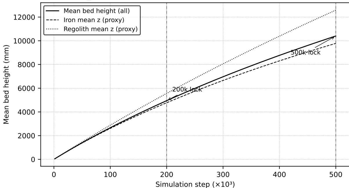
FIG. 7 — Rung 5 sensitivity GPU DEM mobilization progression 0.14 bar rep ( U_G=0.066 m/s); combined degradation; 100.0% contained all ckpts
