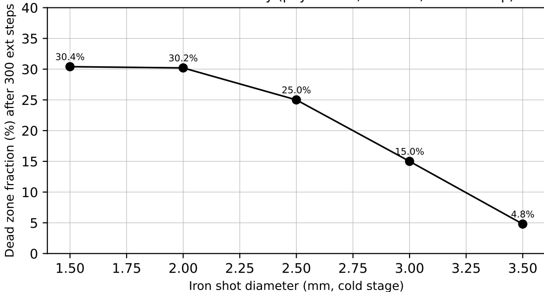
FIG. S1 — Iron size sensitivity (physical lid, N=6500, 0.14 bar rep)
