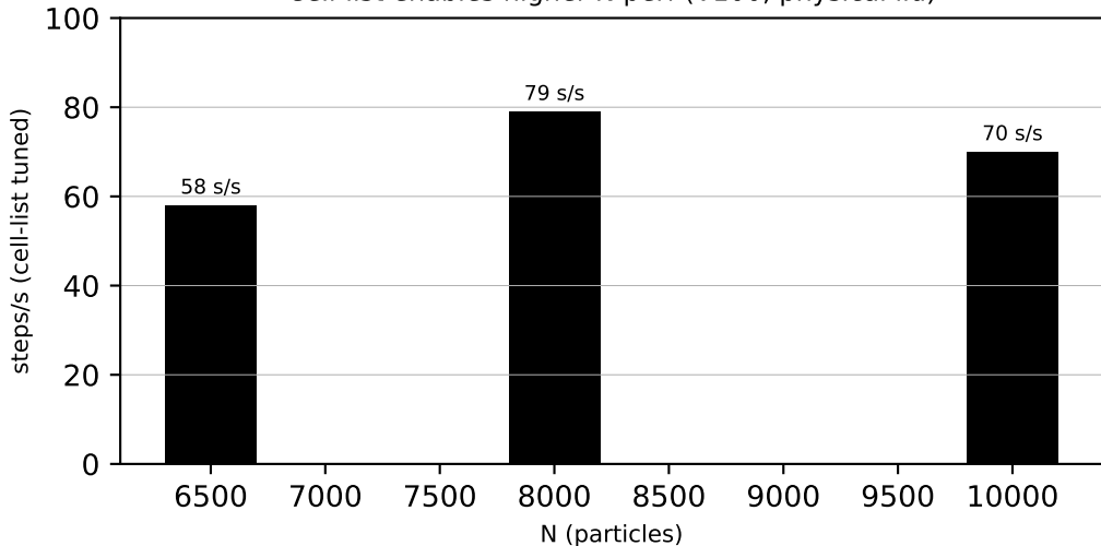
Cell-list enables higher-N perf (V100, physical lid)
