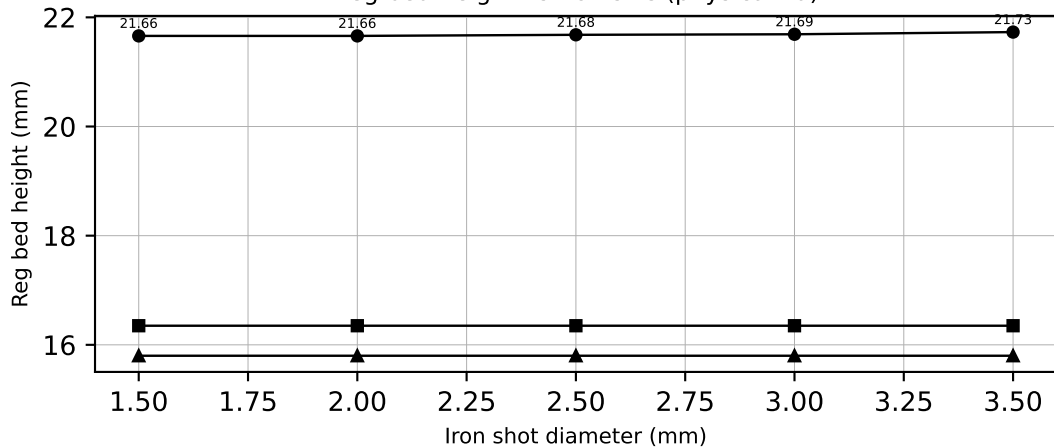
Reg bed height vs iron size (physical lid)
