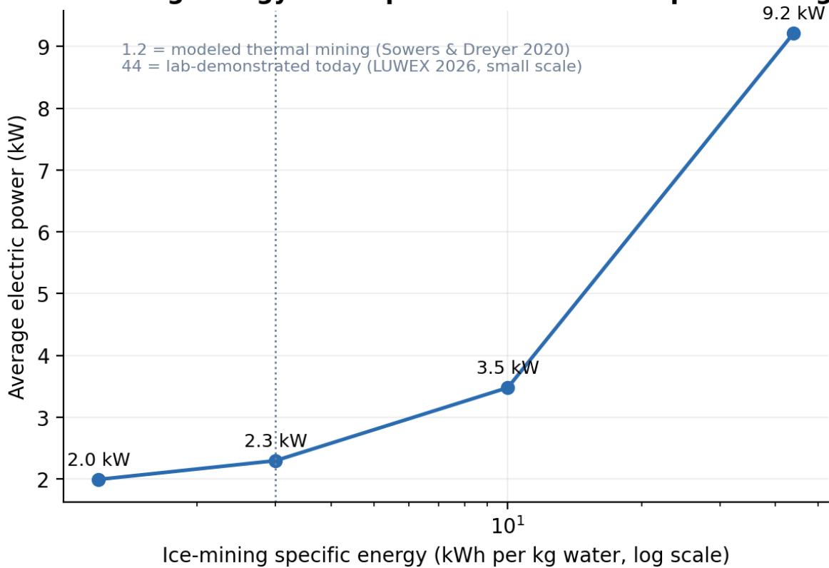
Figure 2 — Plant power vs ice-mining specific energy.
