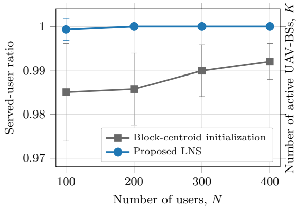
(a) Served-user ratio
