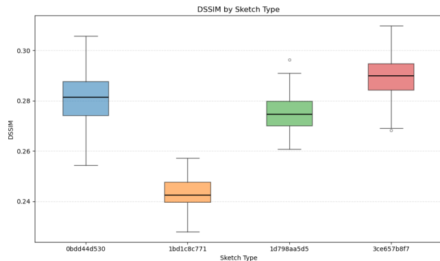
FIGURE 11. Box plot of DSSIM values for sketches groups.
