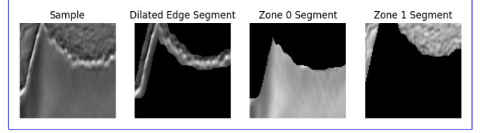
FIGURE 6. Real seismic saline images divided by context zones as input to the texture synthesis process.
