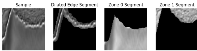
FIGURE 6. Real seismic saline images divided by context zones used as input to the texture synthesis process.
