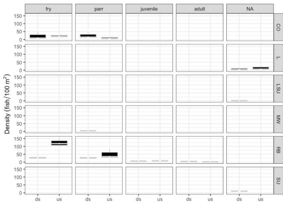
Figure 5.22: Densities of fish (fish/100m²) captured upstream and downstream of PSCIS crossing 197662.
