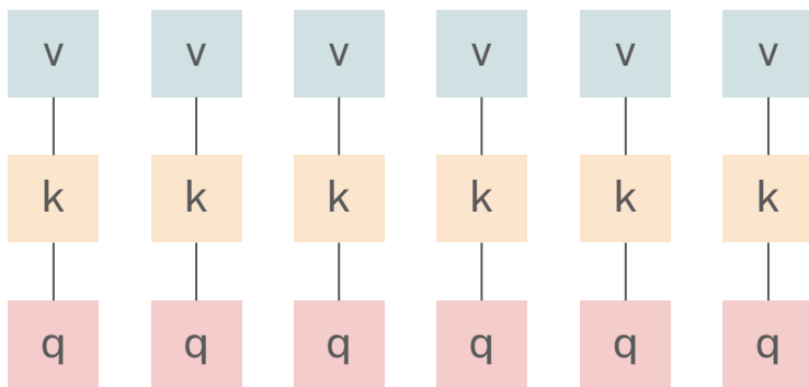
Multi-head attention
