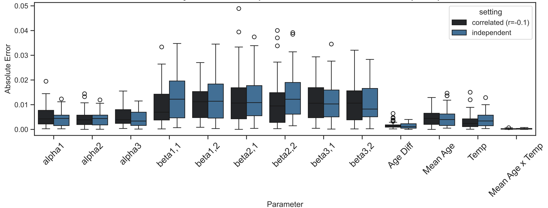
Absolute Error by Parameter, Independent vs Correlated Innovations ( r=-0.1 ): ER
