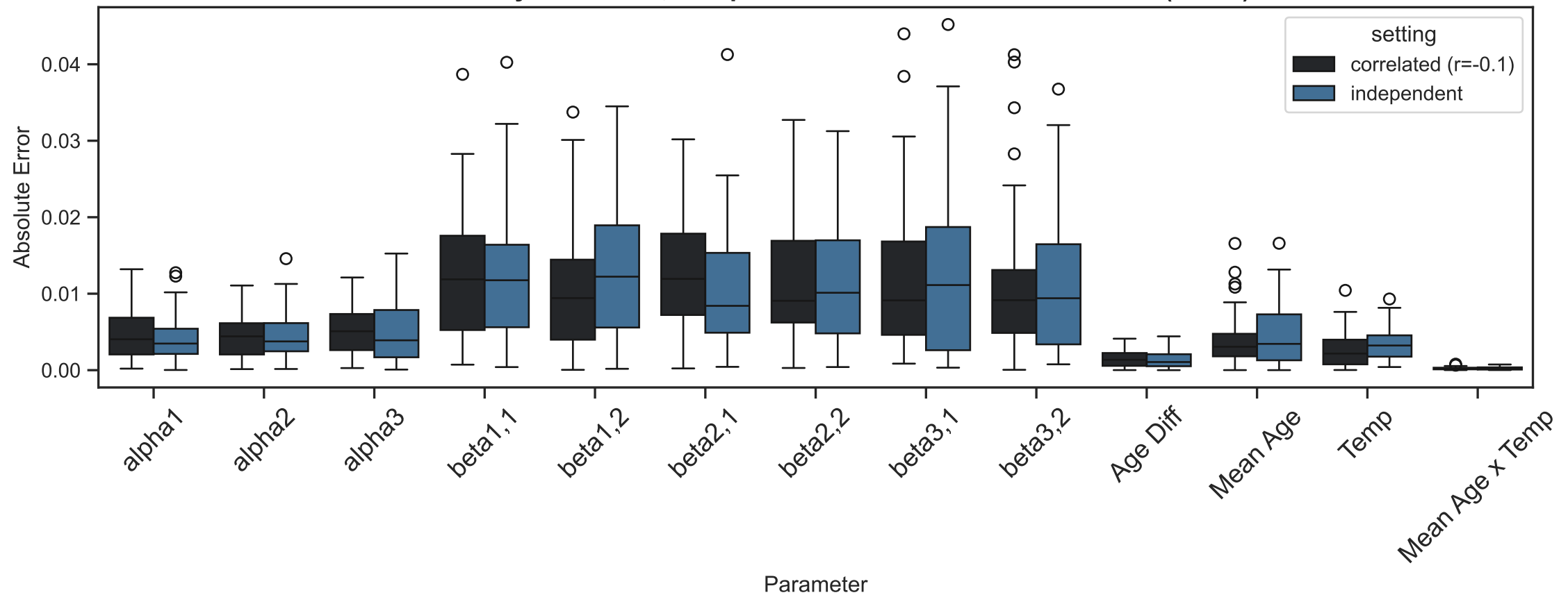
Absolute Error by Parameter, Independent vs Correlated Innovations ( r=-0.1 ): RDP
