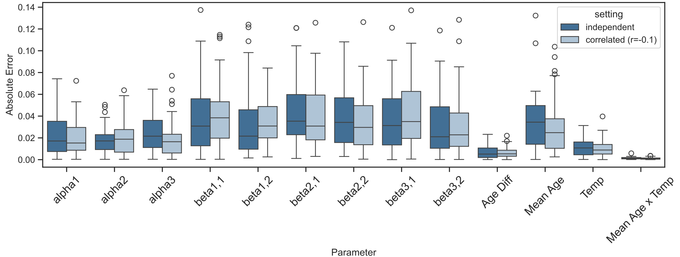
Absolute Error by Parameter, Independent vs Correlated Innovations ( r=-0.1 , 13 nodes): ER
