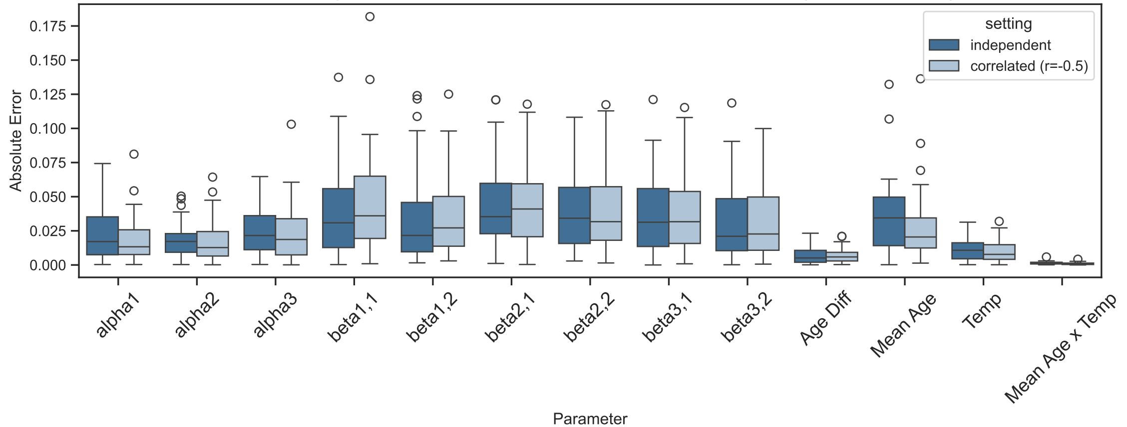
Absolute Error by Parameter, Independent vs Correlated Innovations ( r=-0.5 , 13 nodes): ER
