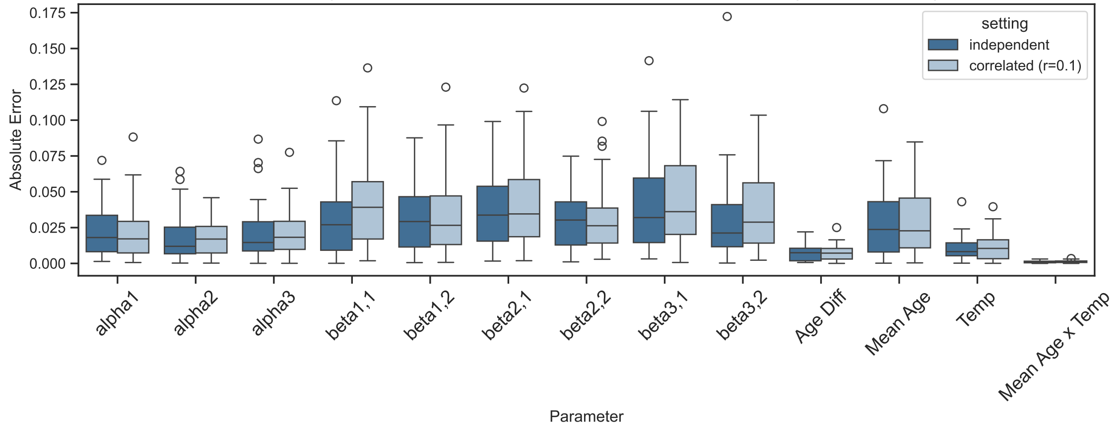
Absolute Error by Parameter, Independent vs Correlated Innovations ( r=0.1 , 13 nodes): RDP
