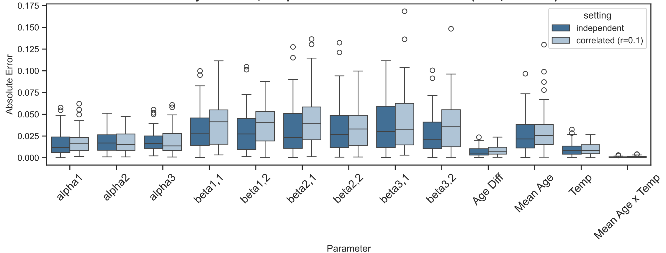
Absolute Error by Parameter, Independent vs Correlated Innovations ( r=0.1 , 13 nodes): SBM
