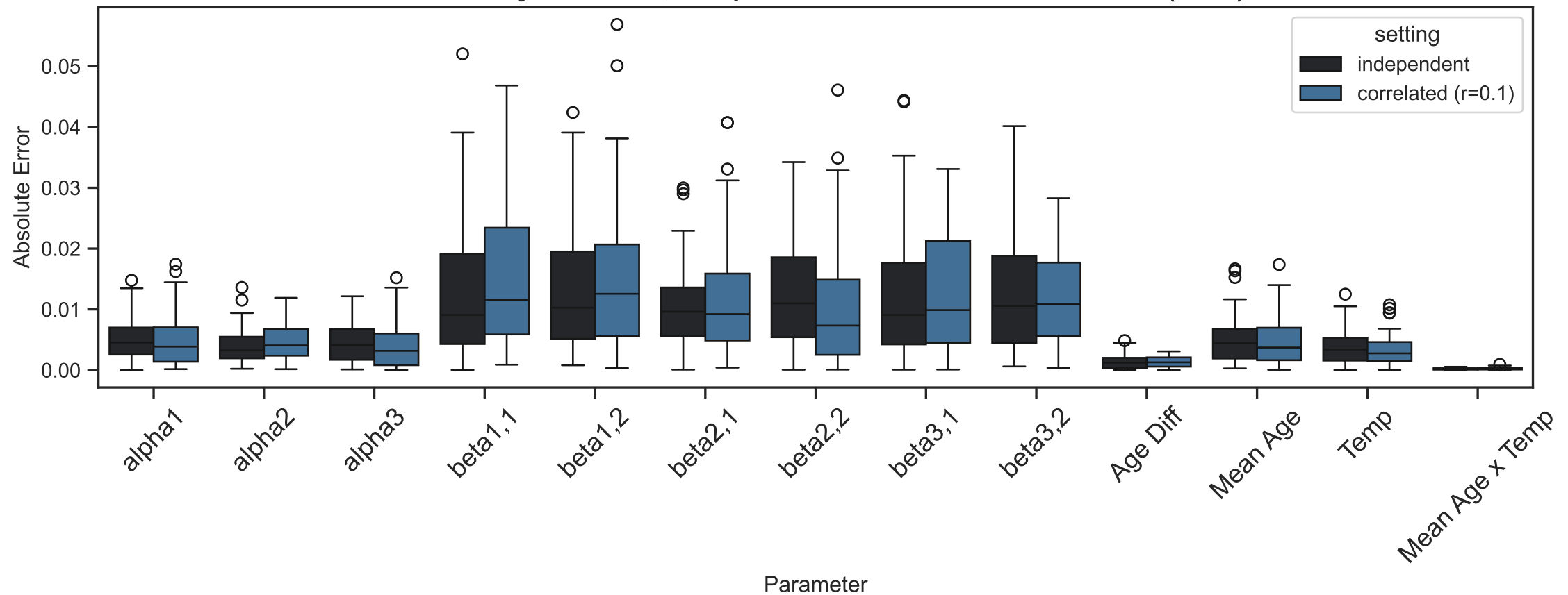
Absolute Error by Parameter, Independent vs Correlated Innovations ( r=0.1 ): SBM
