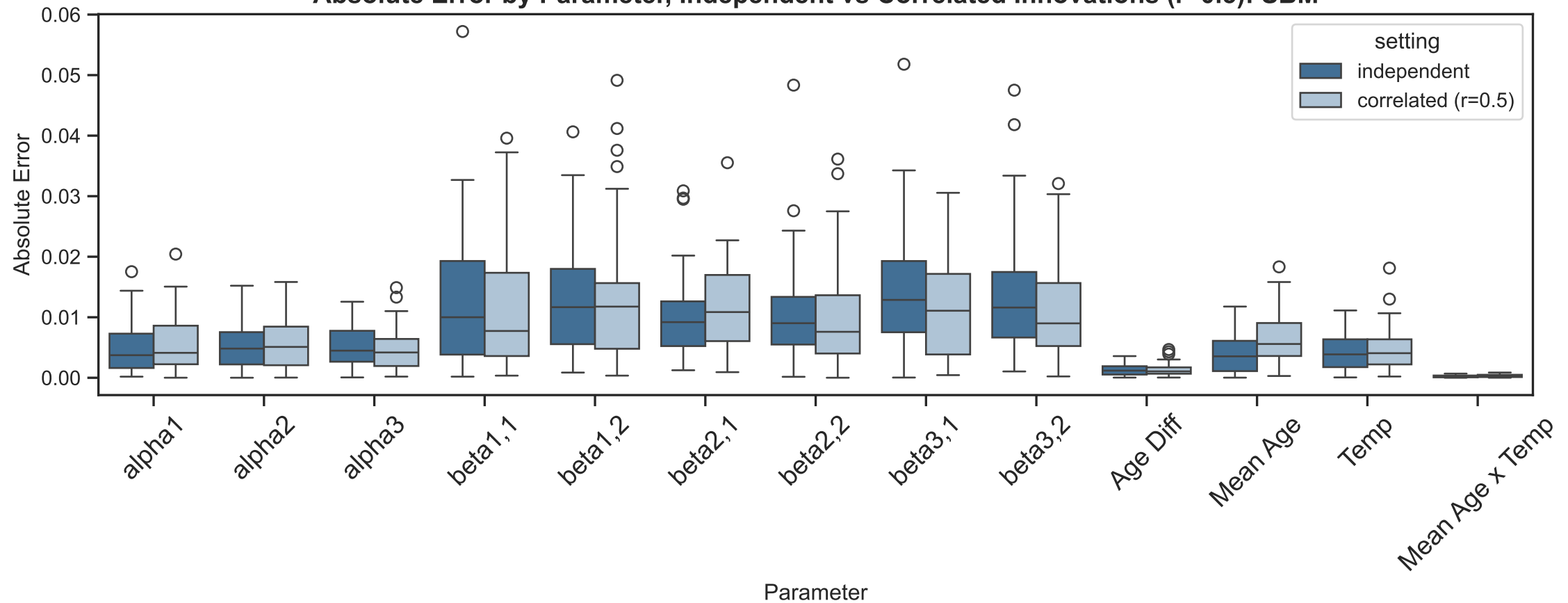
Absolute Error by Parameter, Independent vs Correlated Innovations ( r=0.5 ): SBM
