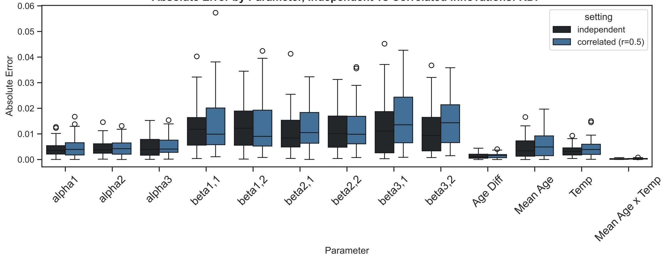
Absolute Error by Parameter, Independent vs Correlated Innovations: RDP
