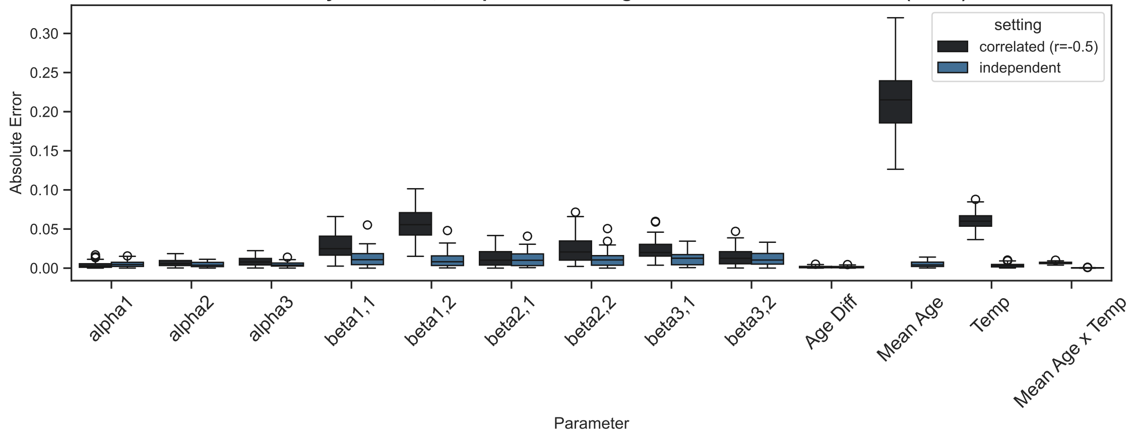
Absolute Error by Parameter, Independent vs Exogenous-Correlated Innovations ( r=-0.5 ): ER
