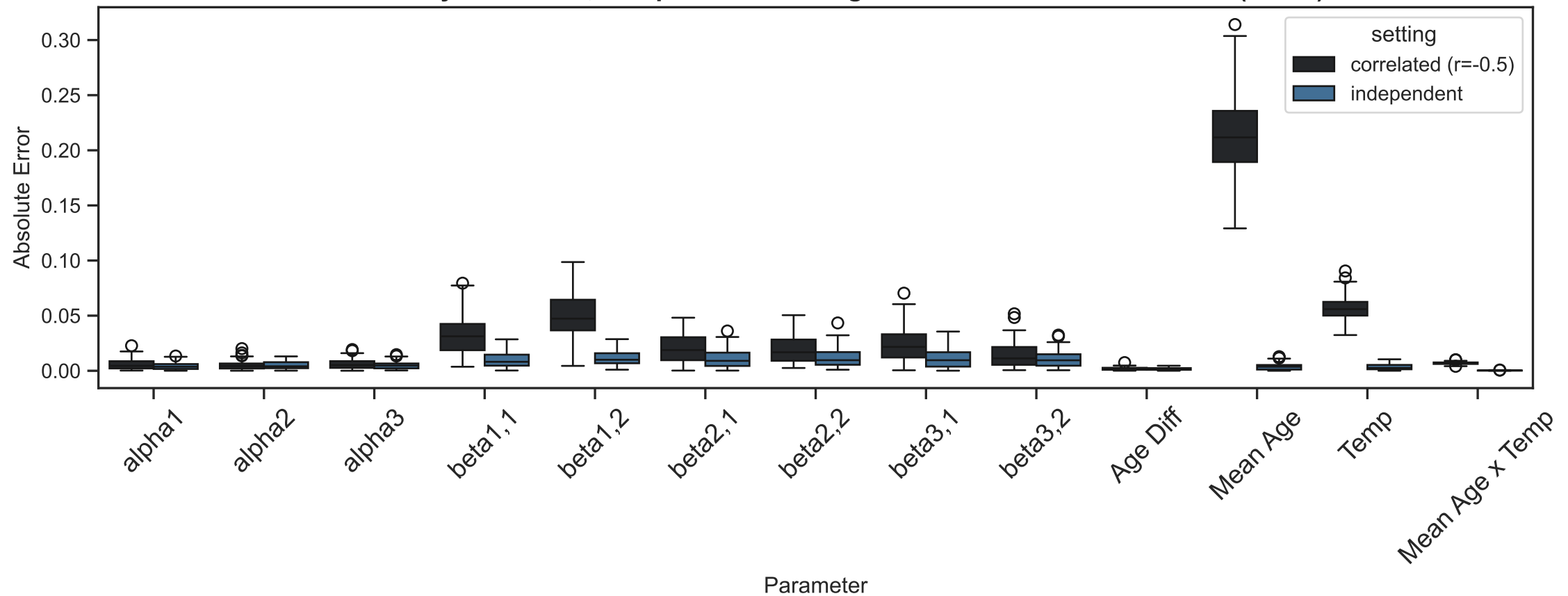
Absolute Error by Parameter, Independent vs Exogenous-Correlated Innovations ( r=-0.5 ): RDP
