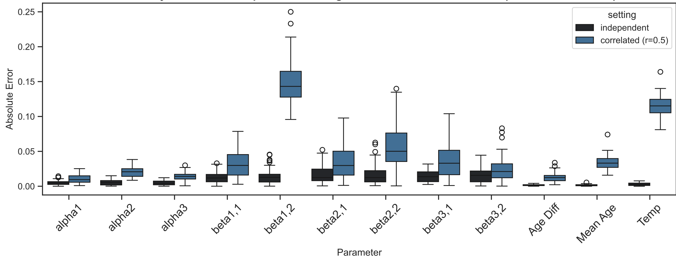
Absolute Error by Parameter, Independent vs Exogenous-Correlated Innovations (No Interaction Term): RDP
