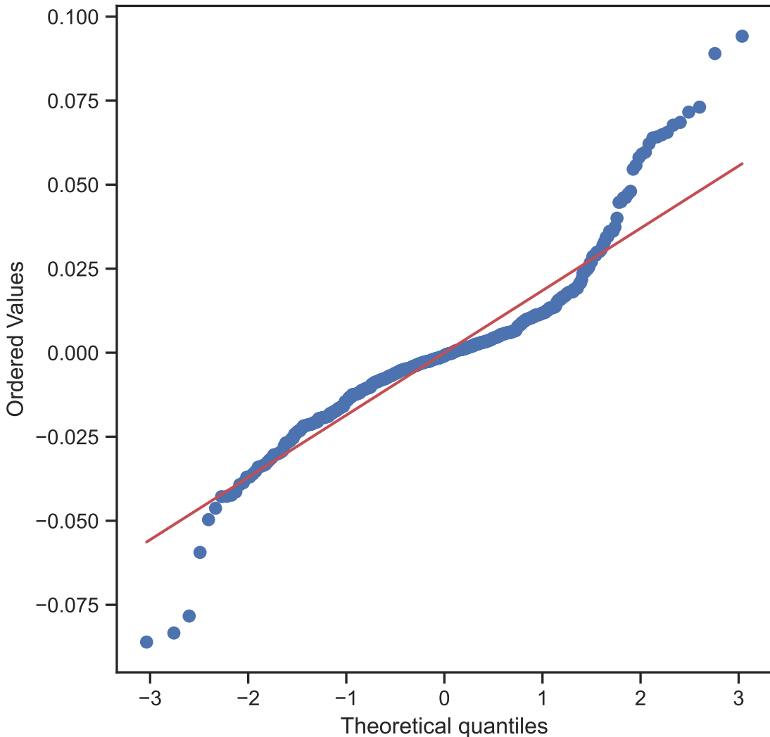
Full model, l = 6 , r = 2 : QQ plot of pooled residuals
