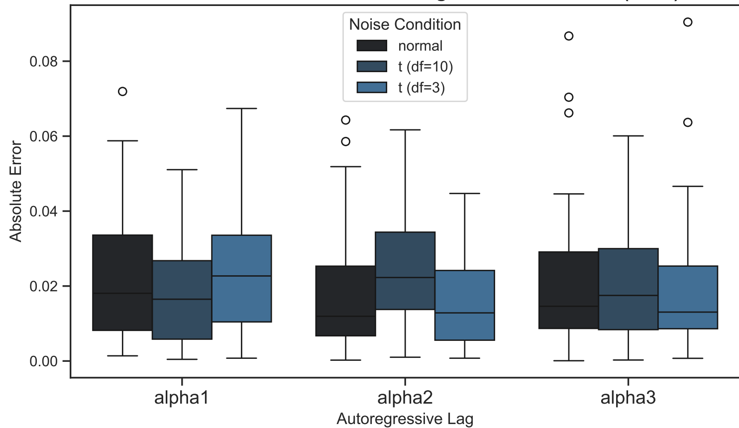
Distribution of Absolute Error for Autoregressive Parameters (K=13): RDP
