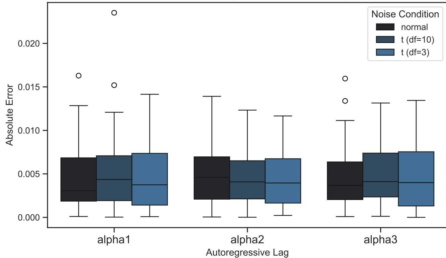
Distribution of Absolute Error for Autoregressive Parameters (No Interaction Term): ER
