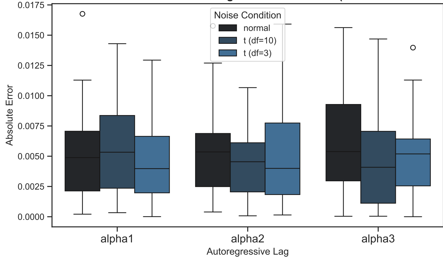
Distribution of Absolute Error for Autoregressive Parameters (No Interaction Term): SBM
