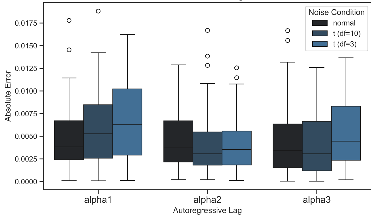
Distribution of Absolute Error for Autoregressive Parameters: SBM
