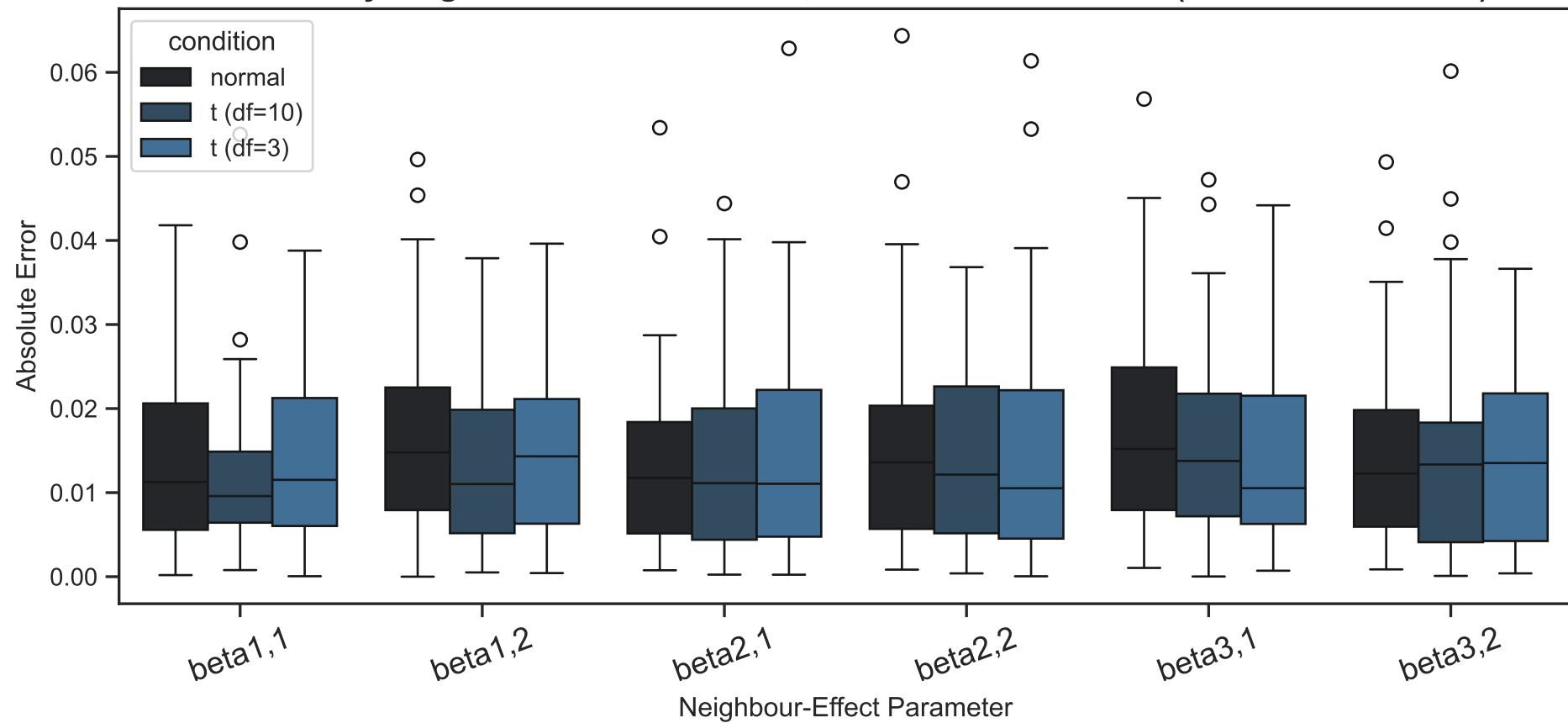
Absolute Error by Neighbour-Effect Parameter, Innovation Distribution (No Interaction Term): RDP
