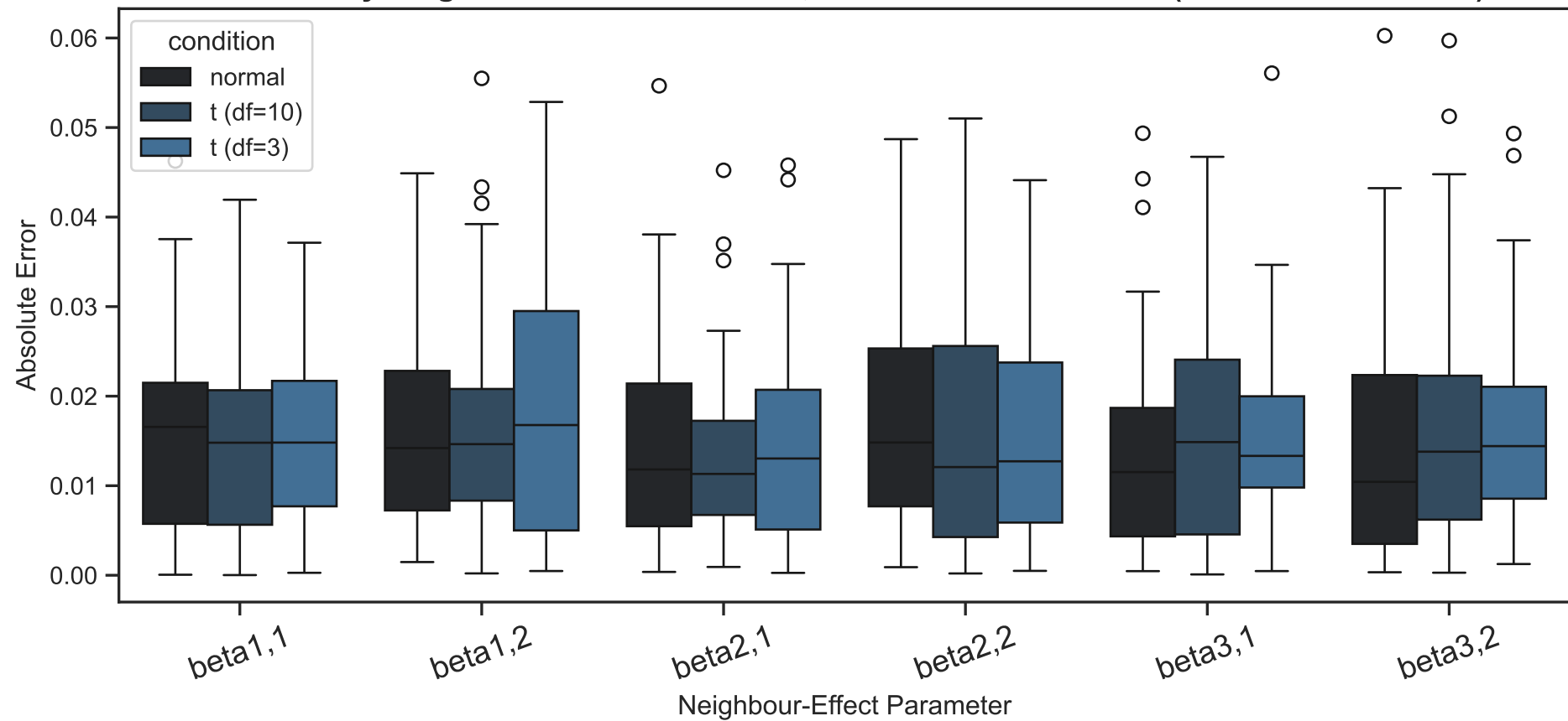
Absolute Error by Neighbour-Effect Parameter, Innovation Distribution (No Interaction Term): SBM
