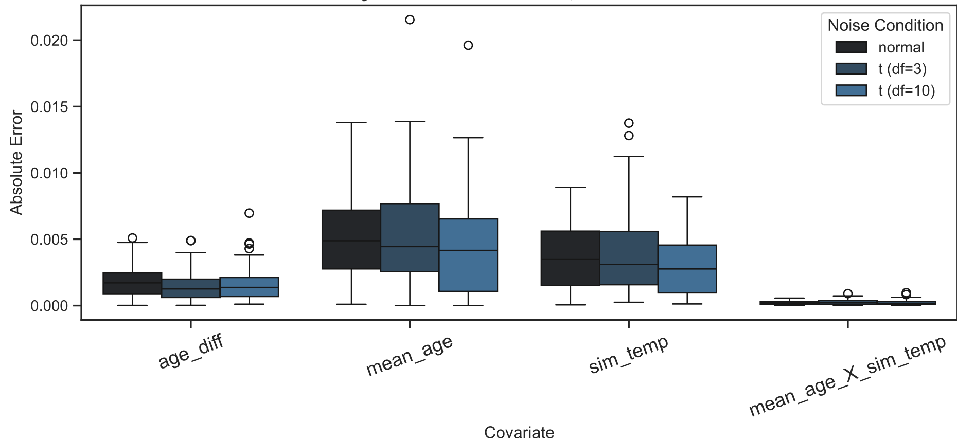
Absolute Error by Covariate Coefficient, Innovation Distribution: ER
