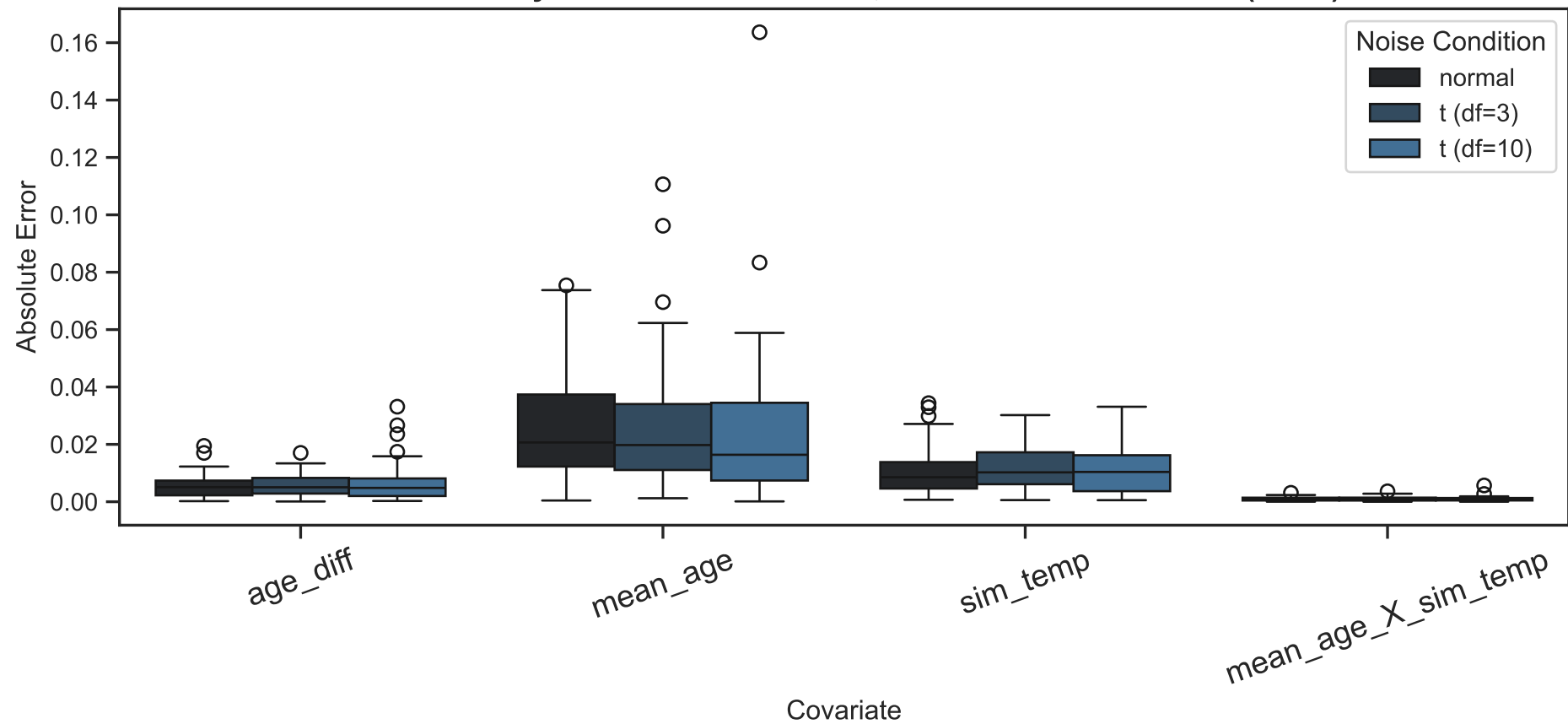
Absolute Error by Covariate Coefficient, Innovation Distribution (K=13): ER
